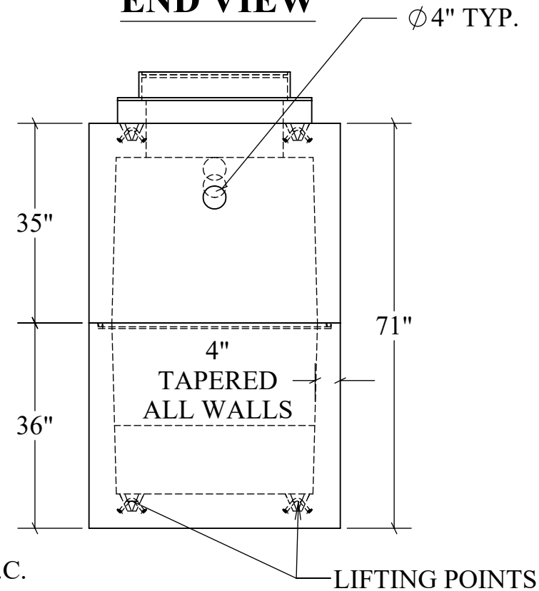
END VIEW
