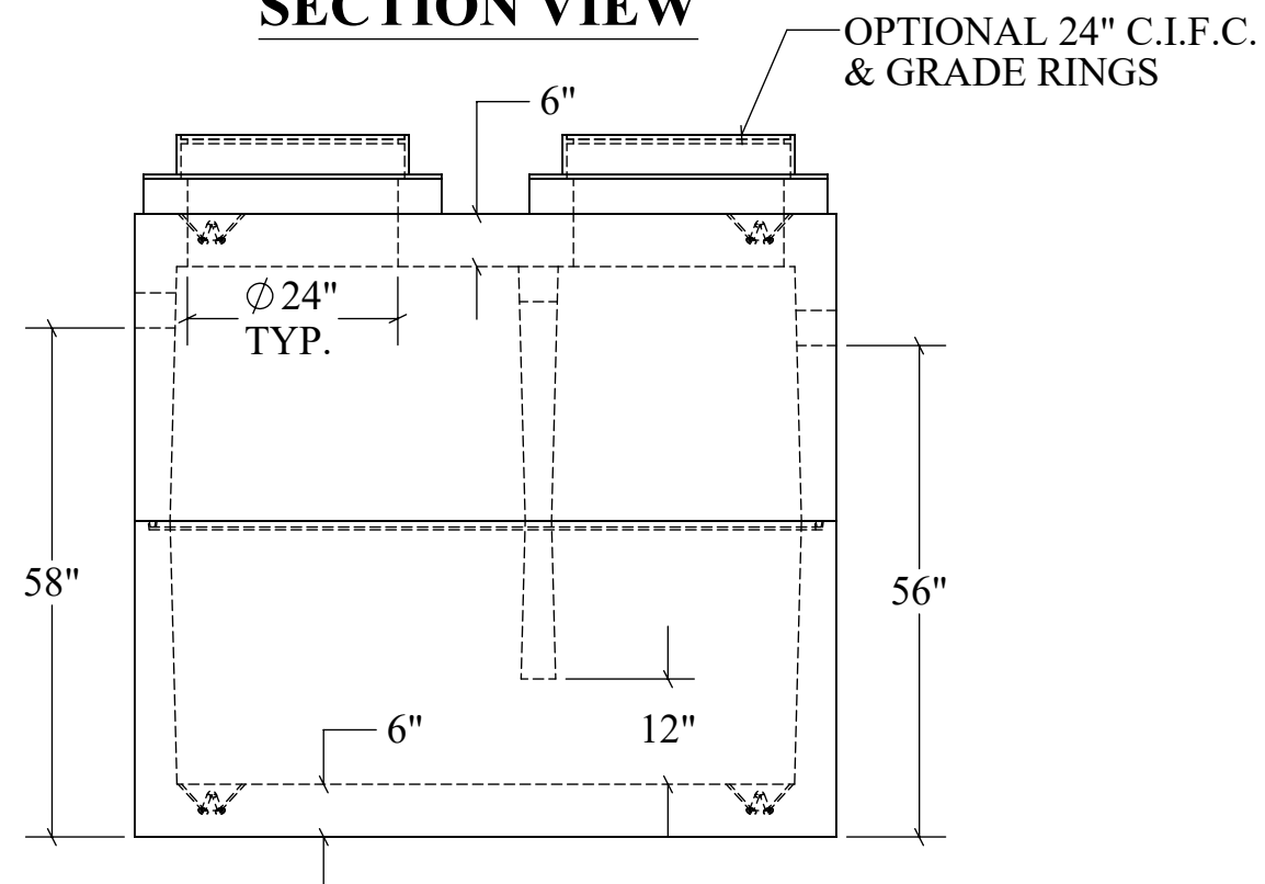
SECTION VIEW
