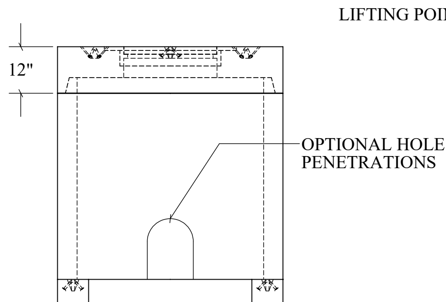
SECTION VIEW
