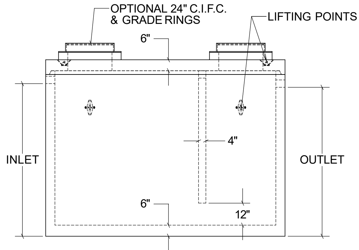
SECTION VIEW
