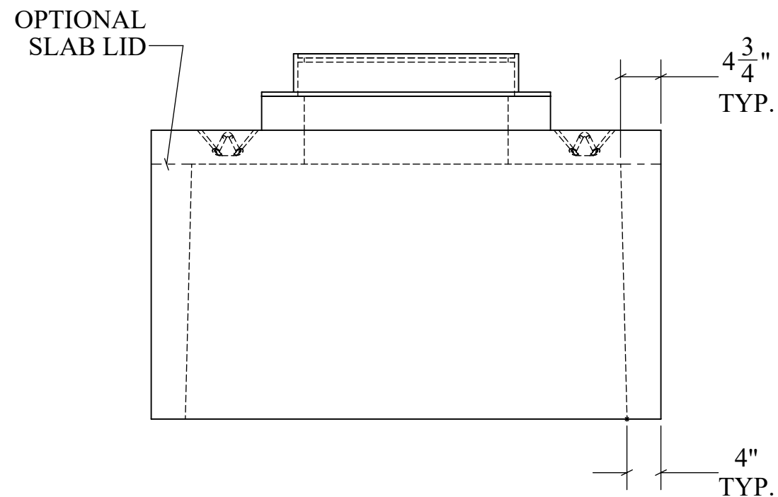
SECTION VIEW
