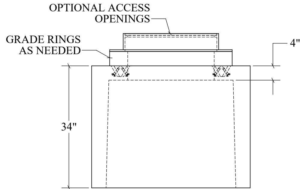
END VIEW
