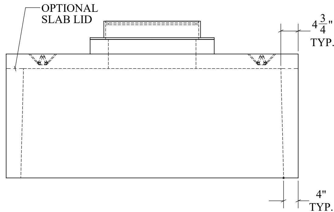
SECTION VIEW
