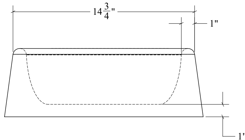
SECTION VIEW
