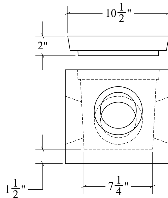
END VIEW
